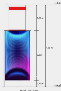
ELEVATION VIEW
